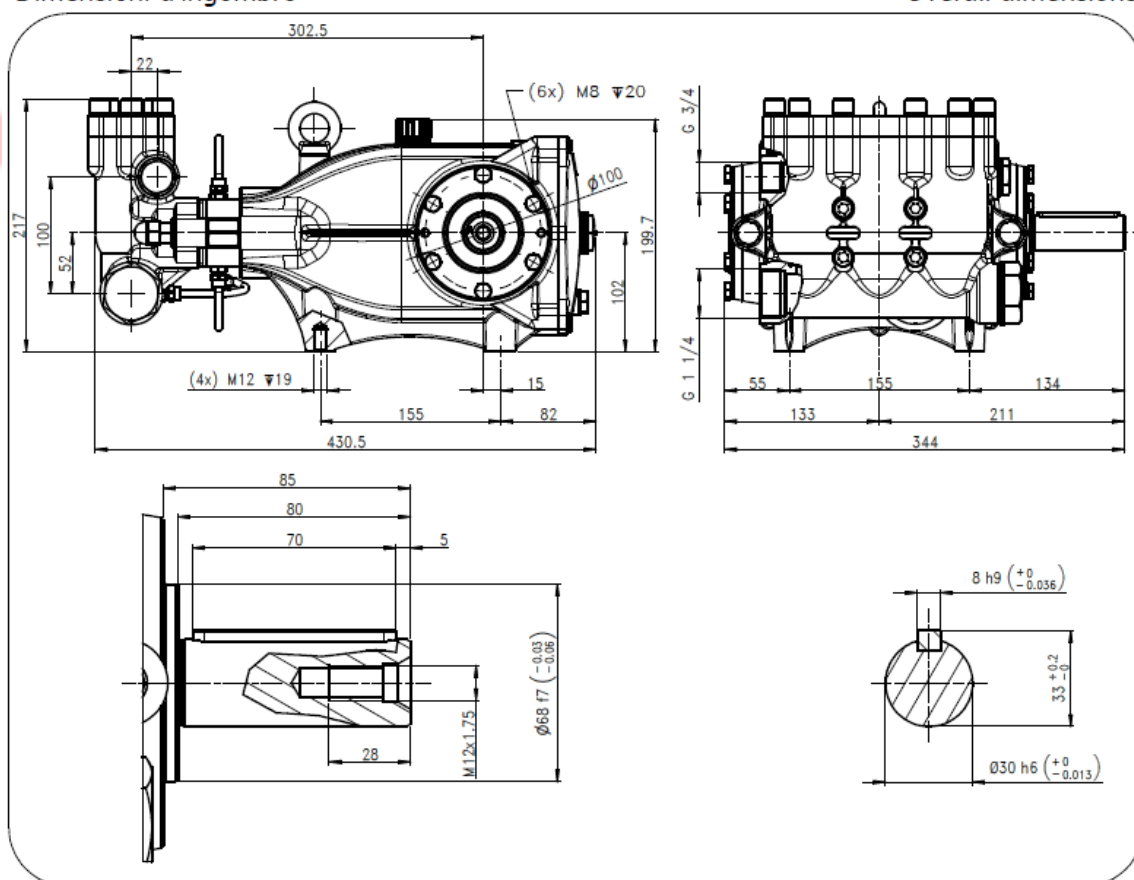
Overall dimensions
